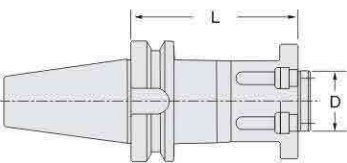
BST 精鏜孔刀頭基礎柄系列 (鏜孔範圍 > Φ200) BST Basic holder for roughness and precision boring bar (Boring range > Φ200)
